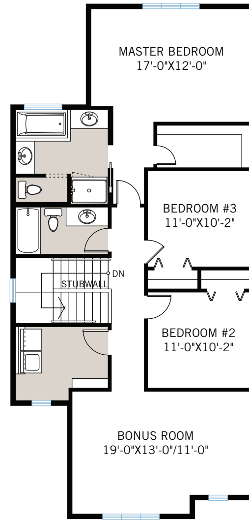
OPTION #16A Alternate Upper Floor - adds 71 sq ft (19 Main, 52 Upper) - Master Bedroom & Ensuite cantilevered out 2'-0"
