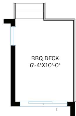
OPTION #9A BBQ Deck - 6'-4"X 10'-0" - 56 sq ft deck
