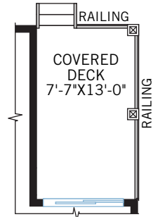
OPTION #9 Covered Rear Deck - adds 99 sq ft
