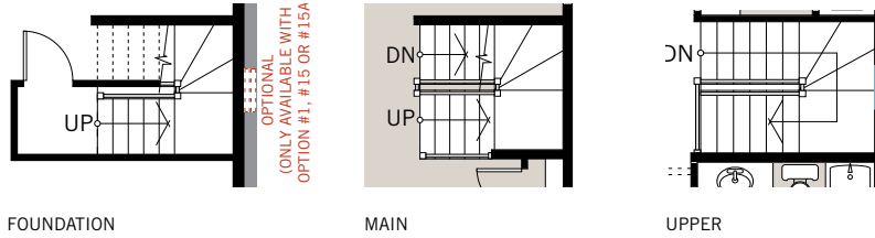
FOUNDATION
