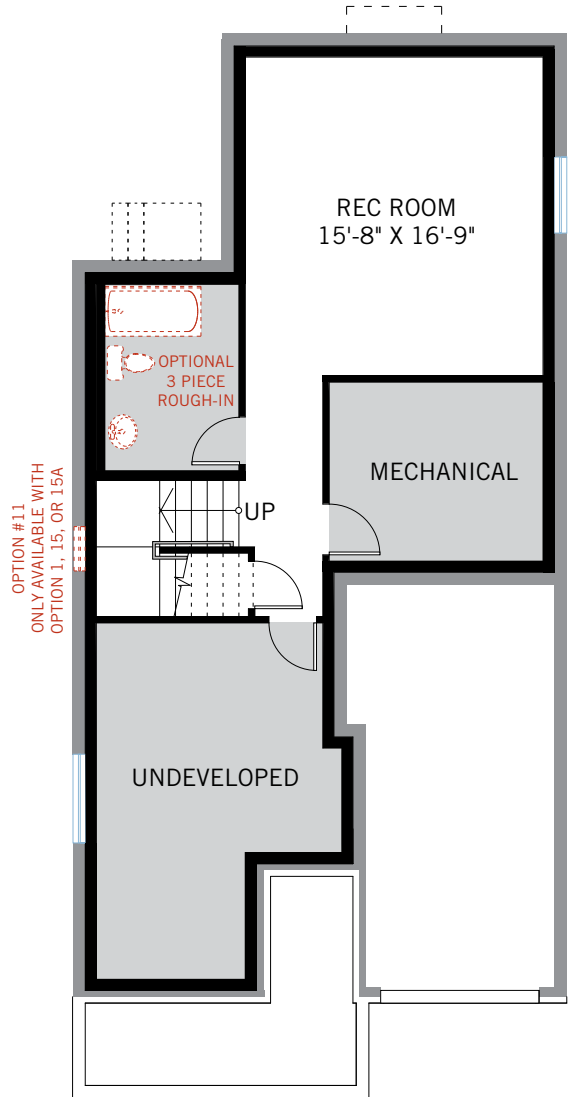
OPTION #15A Developed Rec Room - adds 462 sq ft
