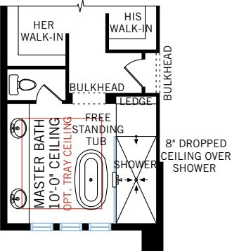
OPTION #8 Upgraded master bathroom
