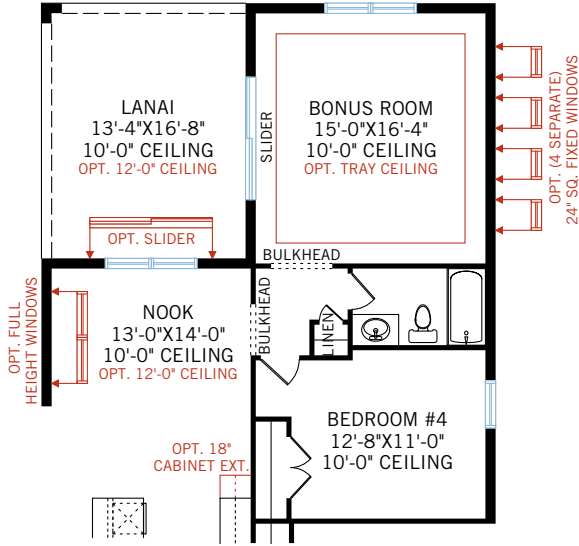
OPTION #3 Bedroom #4 with additional bonus room and lanai - adds 272 sq ft to living space - additional Lanai is 222 sq ft
