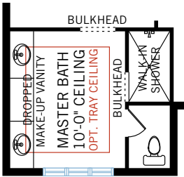
OPTION #5 Extended master bathroom countertops with vanity space - bathtub removed - 24" tall transom windows
