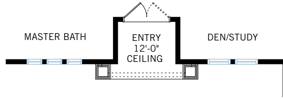
CRAFTSMAN ENTRY 70 sq ft
