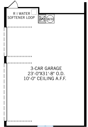
OPTION #4 3-car garage - adds 230 sq ft to garage
