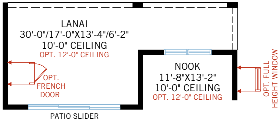
OPTION #2 Extended lanai - adds 185 sq ft
