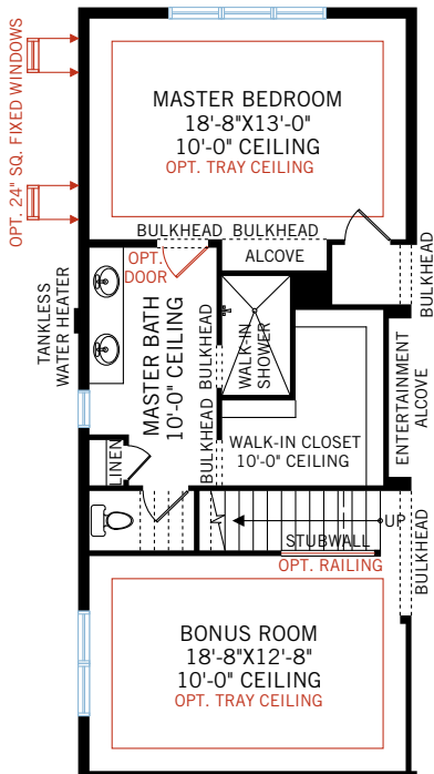
OPTION #4 Upper floor bedroom and bonus room - main floor layout
