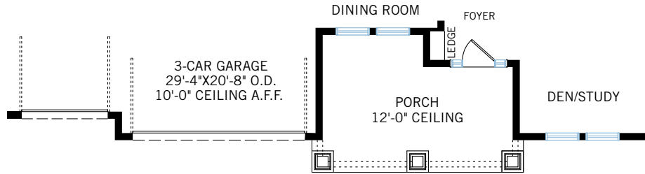
CRAFTSMAN ENTRY 207 sq ft
