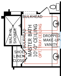
OPTION #6 Extended master bathroom countertops with vanity space - bathtub removed - 24' tall transom windows
