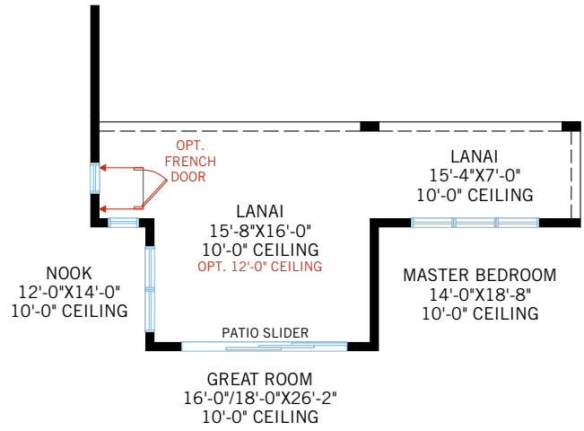
OPTION #2B Extended lanai with rear master lanai - adds 245 sq ft
