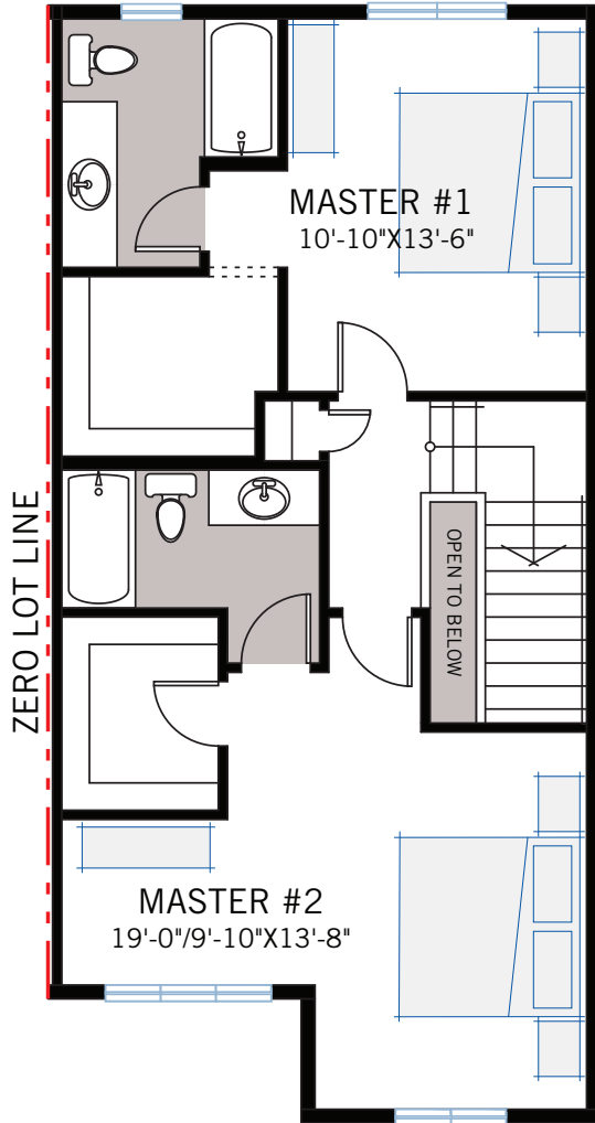
OPTION #16A Alternate Upper Floor Layout - no additional sq ft
