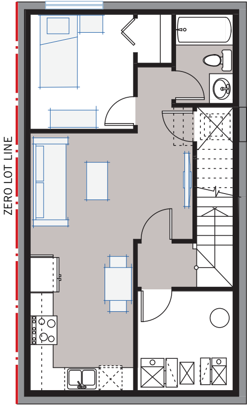
SECONDARY SUITE CONCEPT 1
