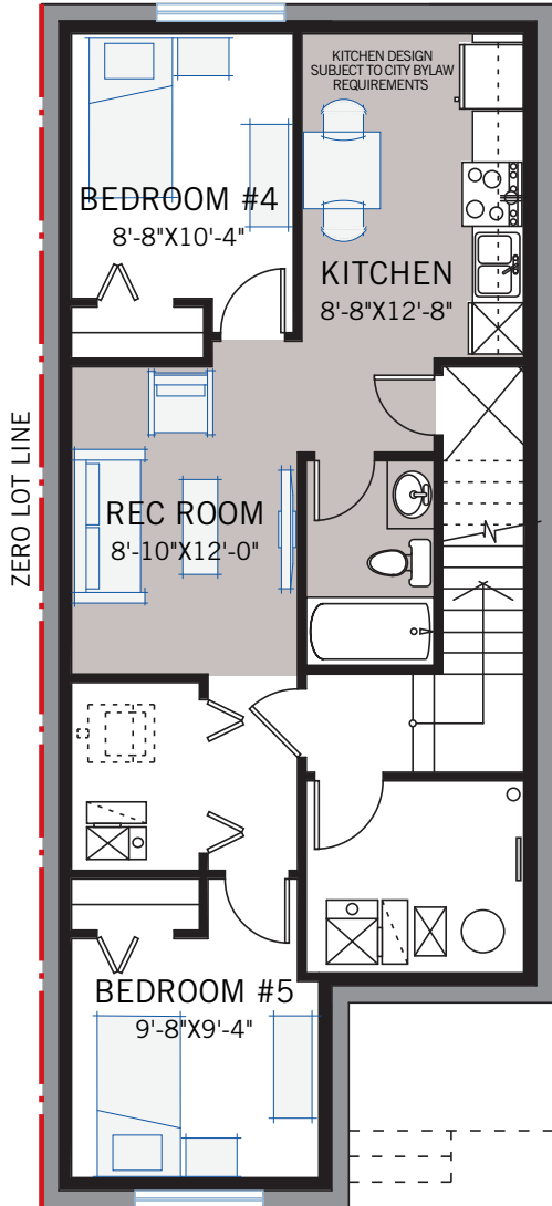
SECONDARY SUITE CONCEPT
