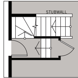
OPTION #05A Exterior Side Entry to Basement - subject to site specific lot grading - undeveloped floor area in basement stairwell - may not be available due to grade constraints
